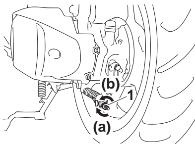
1. Rear brake lever free play adjusting nut
