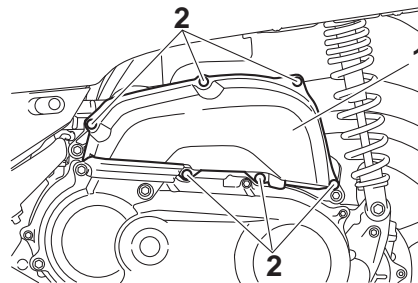
1. Air filter case cover 2. Screw
