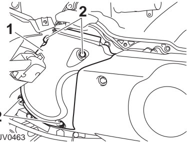
1. V-belt case air filter element cover 2. Bolt
