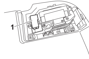
1. Fuse box
